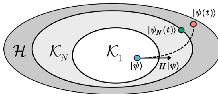
Schematic of Krylov Approximation Method
